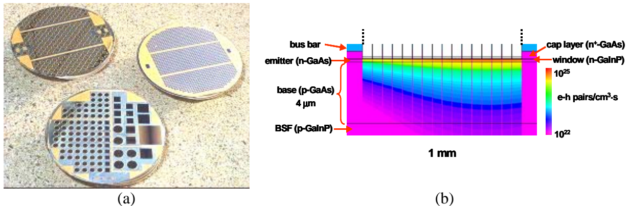
Fig. 1 (a) Dual junction solar cells in their wafer. (b) computer simulation of the photogenerated current in a concentrator solar cell under non uniform illumination.
